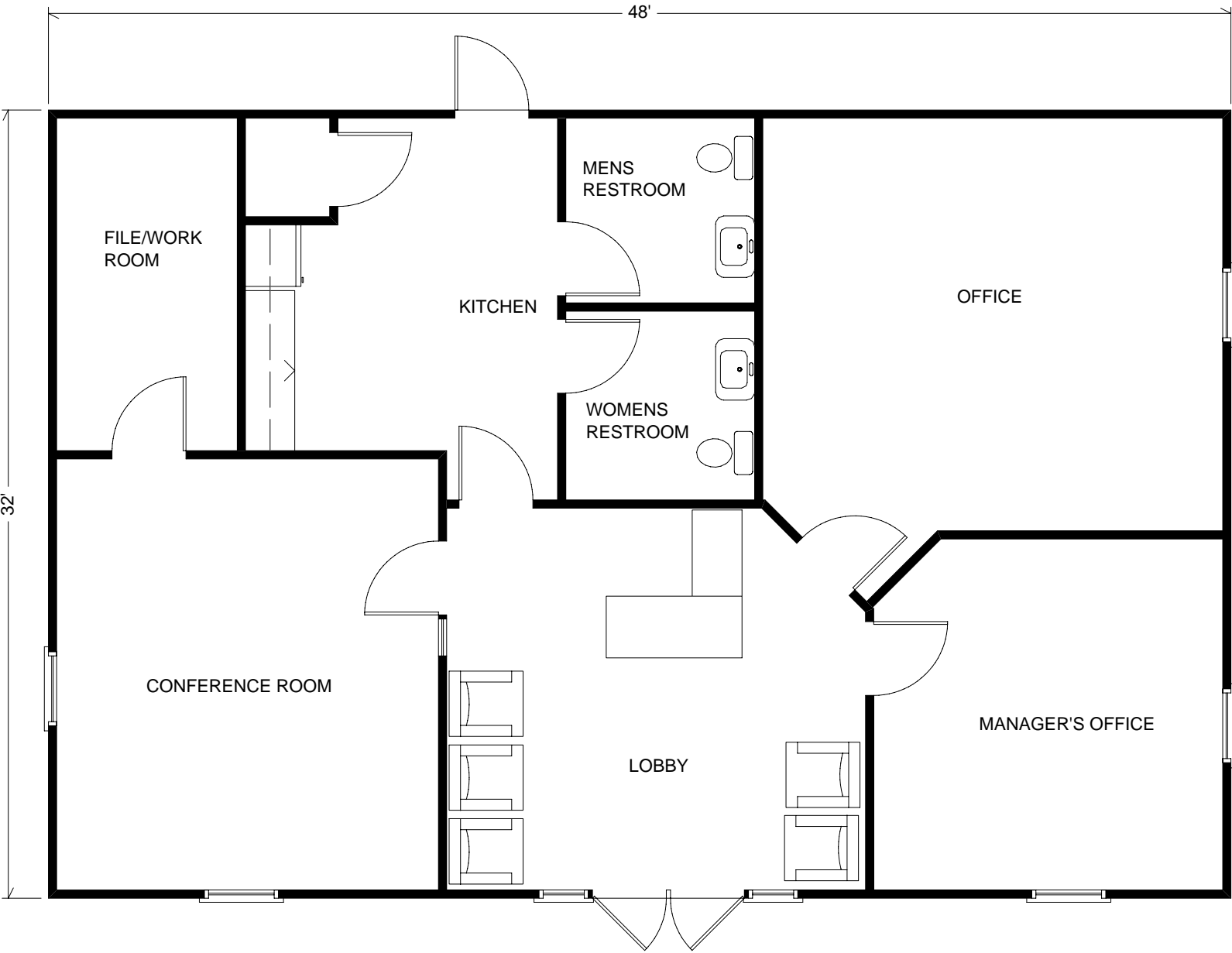
32' X 48' Office Building KC Modular, LLC. Copyright 2008
